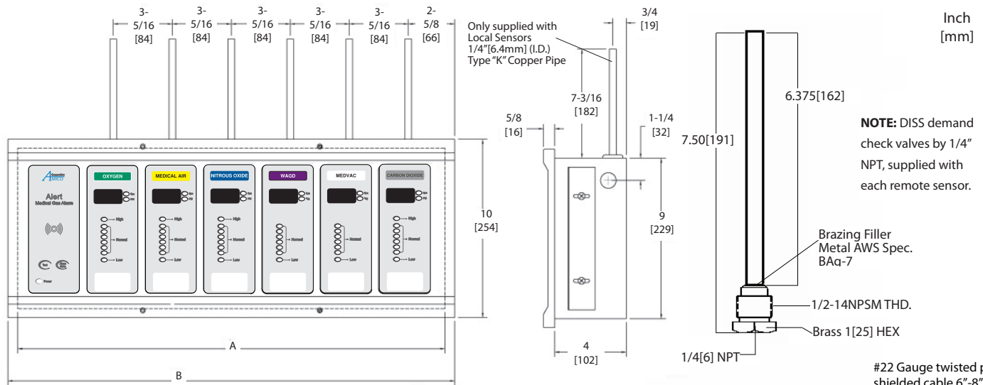
1 module = A2AL-E-X 2 gang back box
