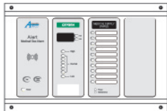
2 modules = A2AL-E-XM 4 gang back box
